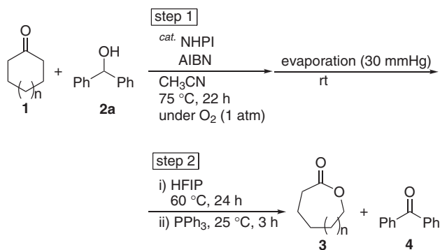
Scheme 1. Baeyer–Villiger oxidation of cycloalkanones 1 with H_2O_2 generated in situ from benzhydrol ( 2a ) and O_2 catalyzed by NHPI/AIBN system.
