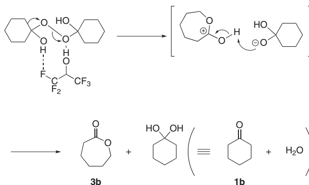
Scheme 3. A possible disproportionation of E ( n = 1) to 1b and 3b induced by HFIP.
