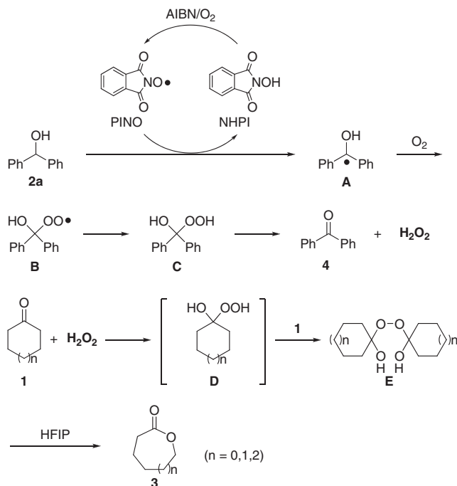
Scheme 2. A possible reaction path for the BV oxidation of 1 with 2a and O 2 by NHPI/AIBN system.
